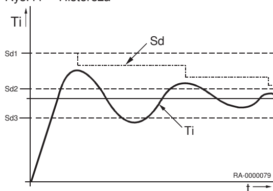
Rys.41 Histereza
